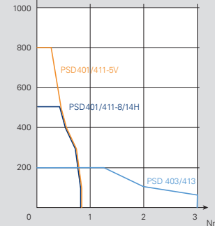
Characteristic curve PSD 40x/41x
